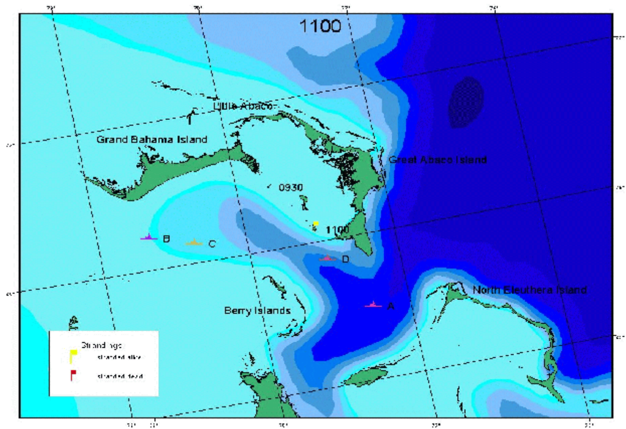
Figure 2c: Map of strandings at 1100 relative to ship positions (ships A-D) when sonars were turned on.
